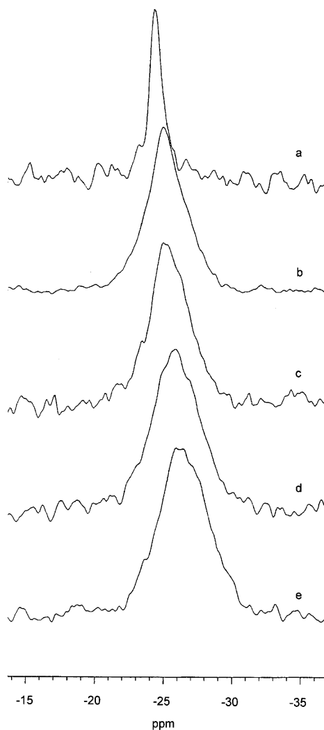
Fig. 4 ^{29}\text{Si} MAS NMR spectra of [\text{Hept Si}(\text{CH}_2)_3\text{OPh}]_n ( 3d ) at different temperatures: a) 40 °C, b) 24.5 °C, c) 15 °C, d) 0 °C, e) -20 °C
