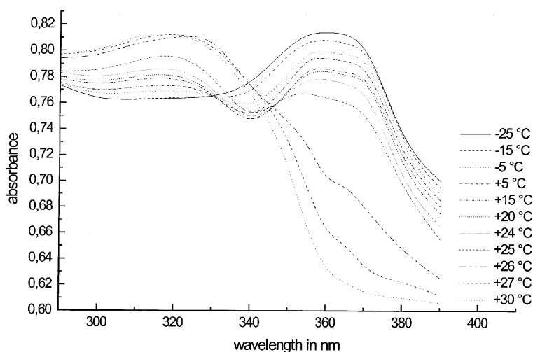
Fig. 3 UV spectrum of [\text{Hept Si}(\text{CH}_2)_3\text{OPh}]_n ( 3d ) as thin film on a quartz plate as function of temperature
